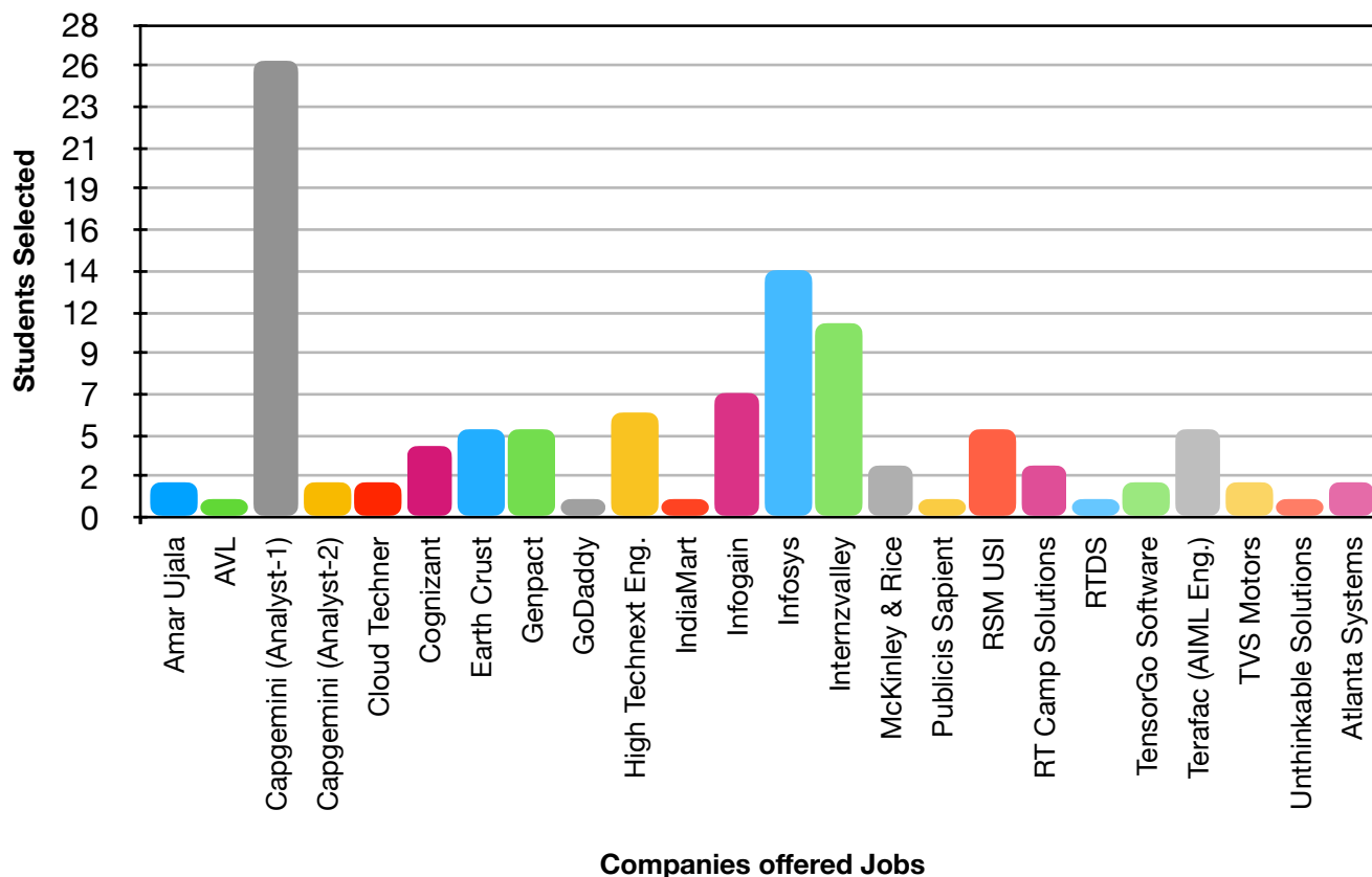
Fig 6: Distribution of Student Selections Across Recruiting Companies
