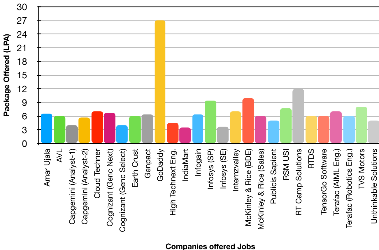
Fig 5: Distribution of Salary-Packages (LPA) for Companies offered jobs
