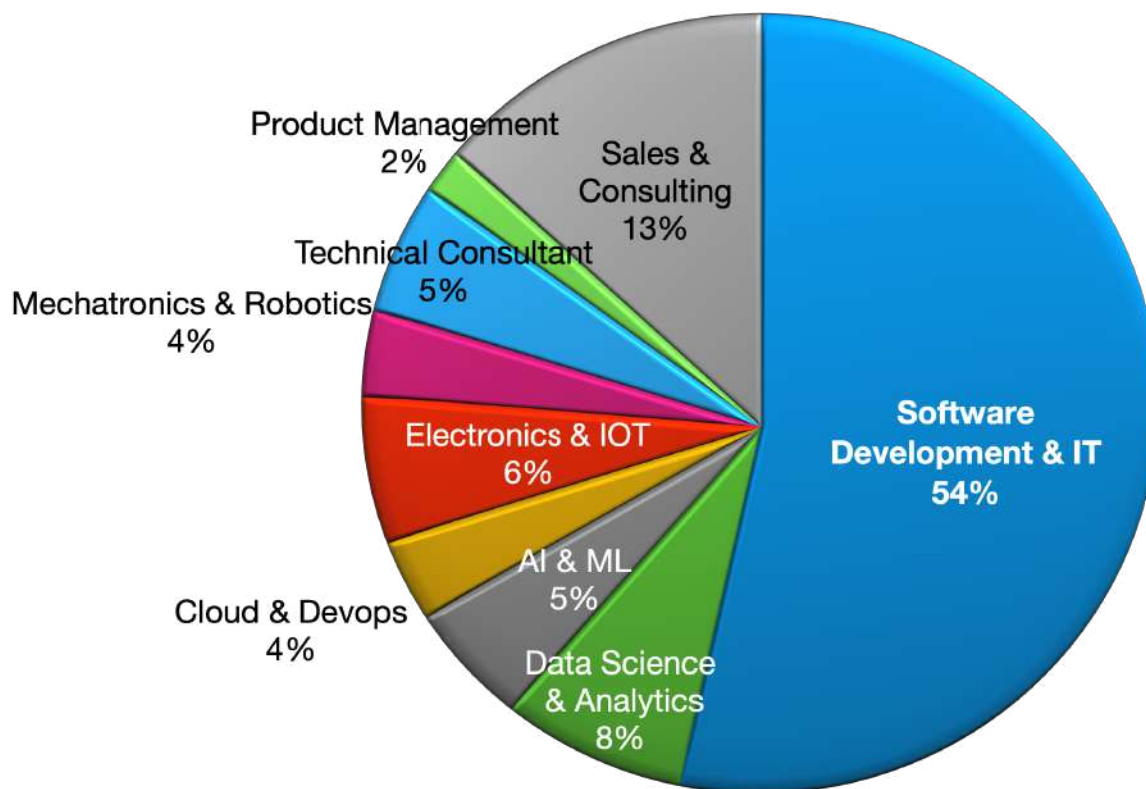
Fig 2: Distribution of Placement & Internship offers in different sectors
