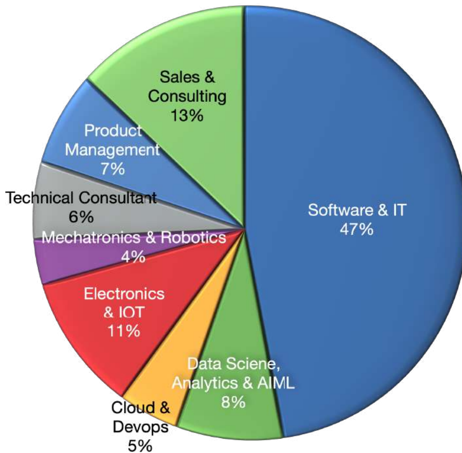
Fig 4: Sector-wise distribution of Companies visited for offering jobs
